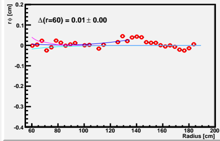
Laser Track at z=-170
