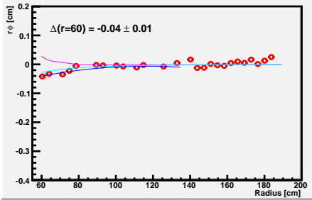
Laser Track at z=-145
