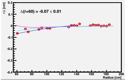
Laser Track at z=-115
