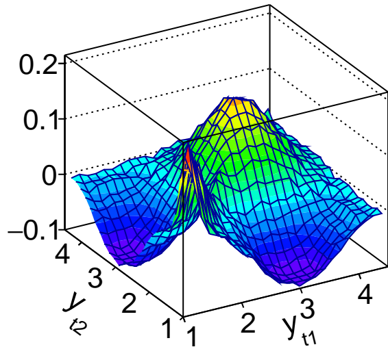
Data All-Cl: 28-38%
