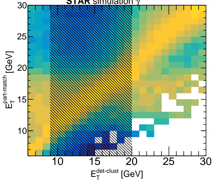
STAR simulation \gamma
