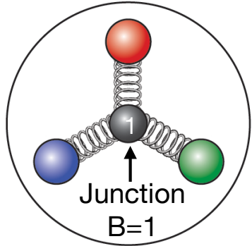
Junctions as baryon carrier
