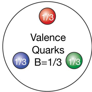
Valence quarks as baryon carrier
