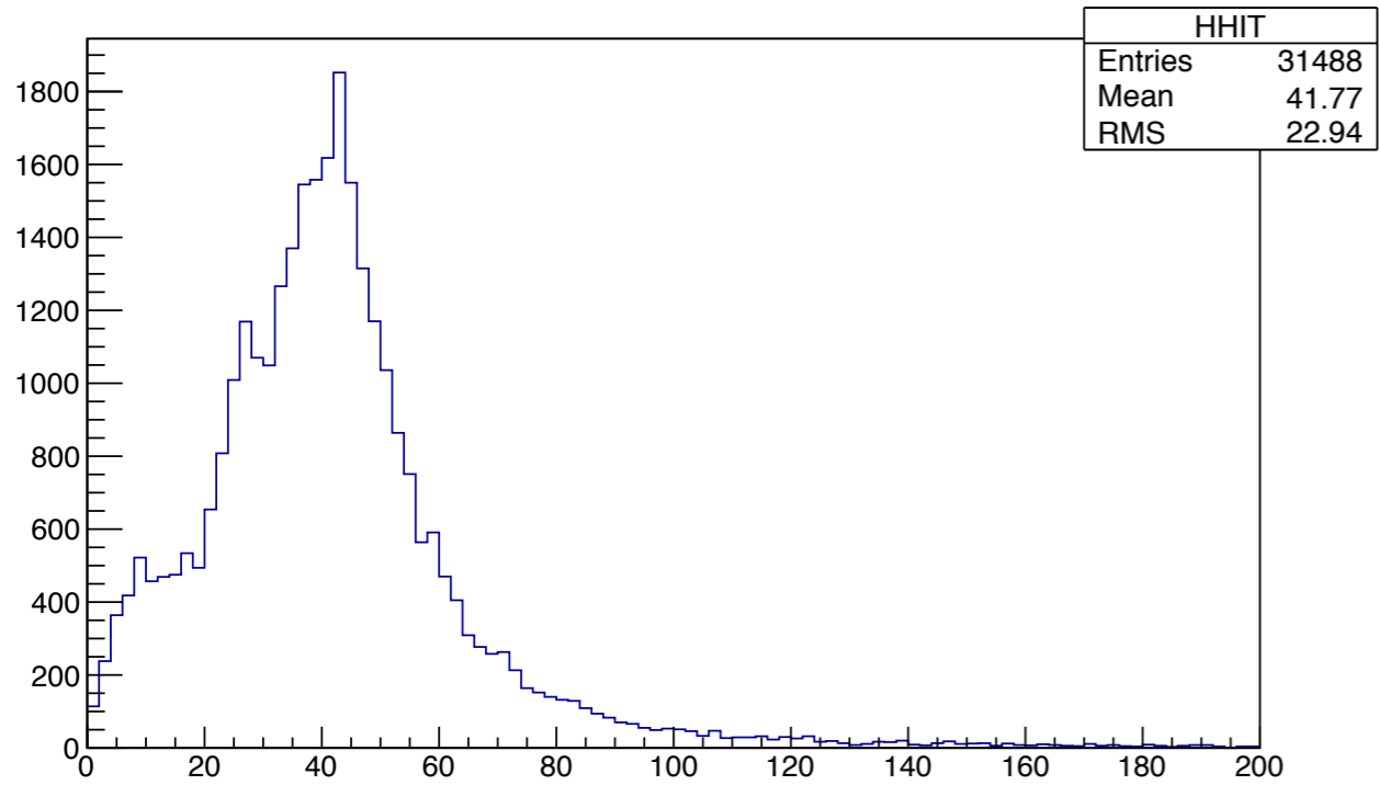
Hit charge distribution
