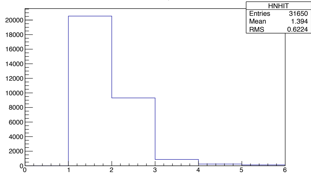
Number of strips in hit
