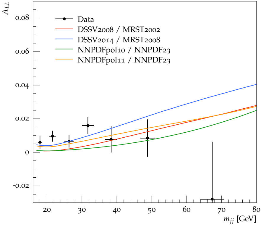
Dijet A_{LL} for |y| < 0.8 , EW+WE, anti- k_T , R = 0.6
