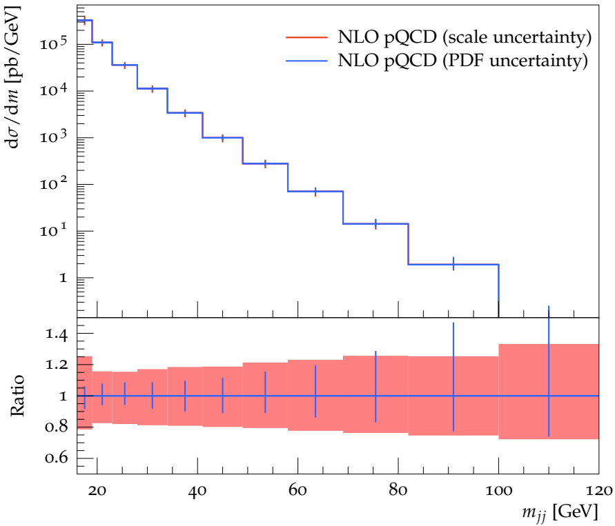
Dijet mass spectrum for |y| < 0.8 , EE+WW, anti- k_T , R = 0.6
