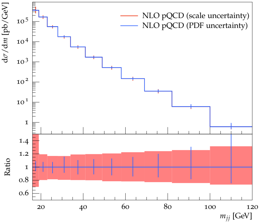
Dijet mass spectrum for |y| < 0.8 , EW+WE, anti- k_T , R = 0.6
