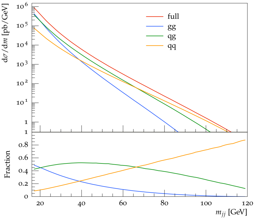
Dijet mass spectrum for |y| < 0.8 , anti- k_T , R = 0.6
