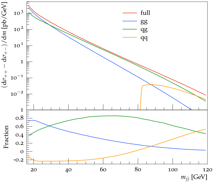
Polarized cross section for |y| < 0.8 , anti- k_T , R = 0.6
