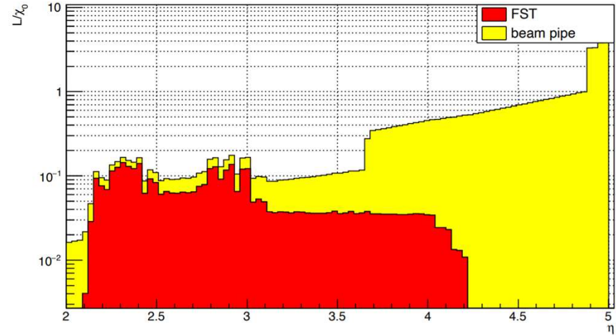
material budget histograms (300 micron)
