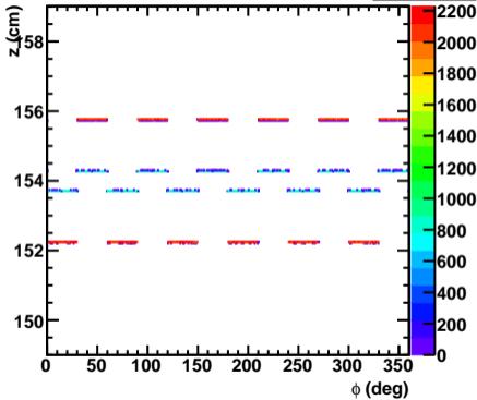
Disk 5 All Sensors
