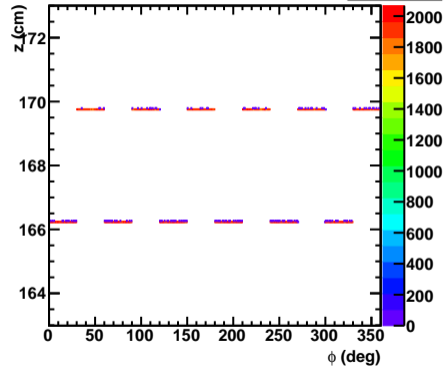
Disk 6 Inner Sensors
