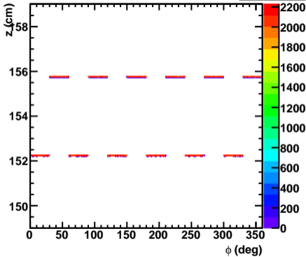
Disk 5 Inner Sensors
