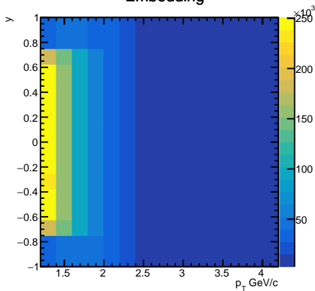
Embedding
