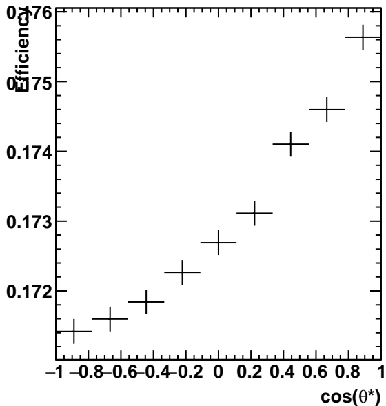
Efficiency 1.2 < p_{\top} < 1.8
