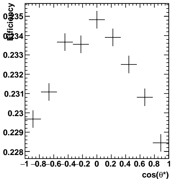
Efficiency 1.8 < p_{\top} < 2.4
