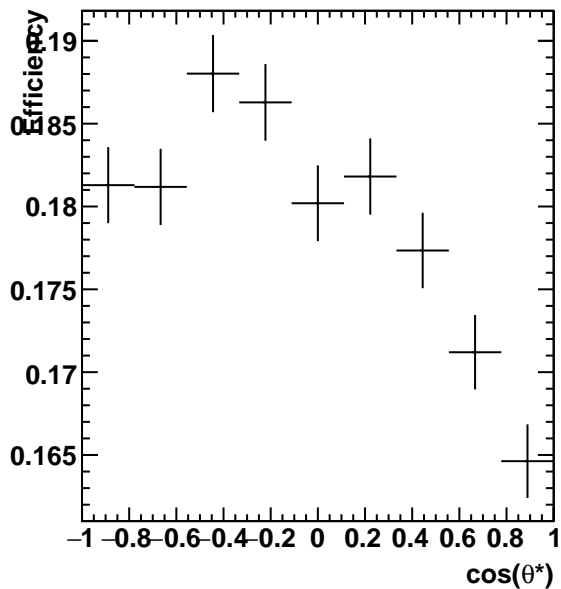
Efficiency 3.0 < p_{\top} < 4.2
