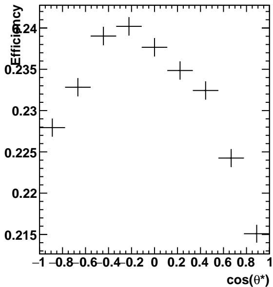
Efficiency 2.4 < p_{\top} < 3.0
