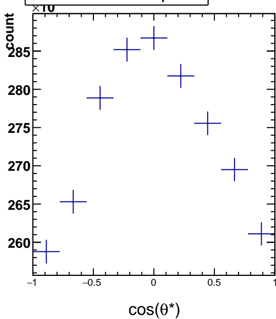
Raw Yields 1.2 < p_T < 1.8
