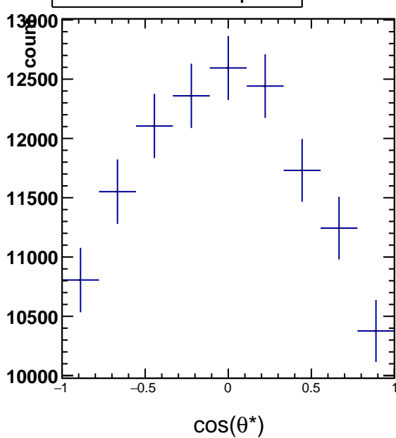
Raw Yields 2.4 < p_T < 3.0
