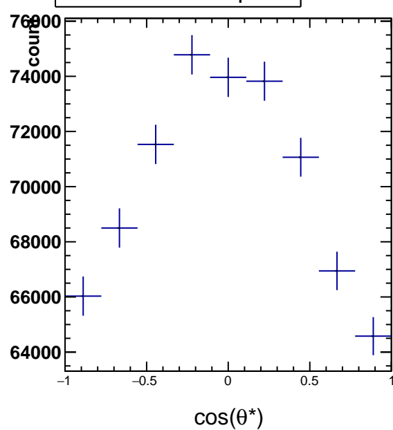
Raw Yields 1.8 < p_T < 2.4
