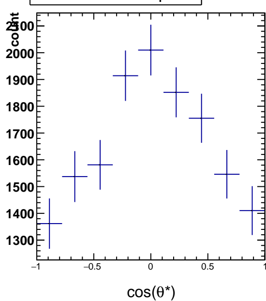
Raw Yields 3.0 < p_T < 4.2
