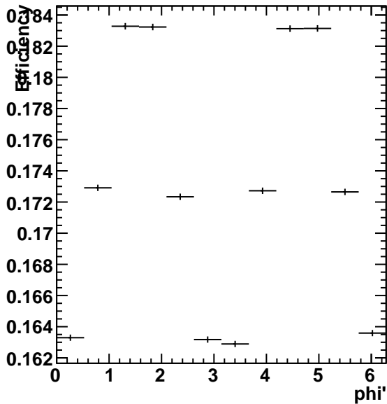
Efficiency 1.2 < p_{\perp} < 1.8
