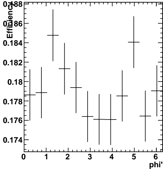
Efficiency 3.0 < p_{\perp} < 4.2
