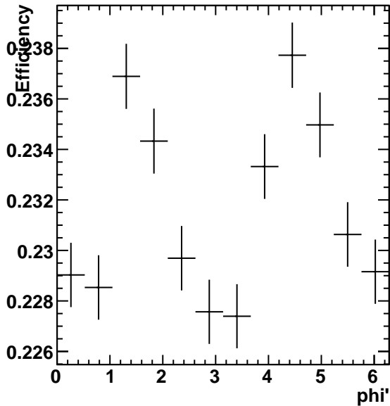
Efficiency 2.4 < p_{\perp} < 3.0
