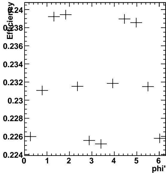
Efficiency 1.8 < p_{\perp} < 2.4
