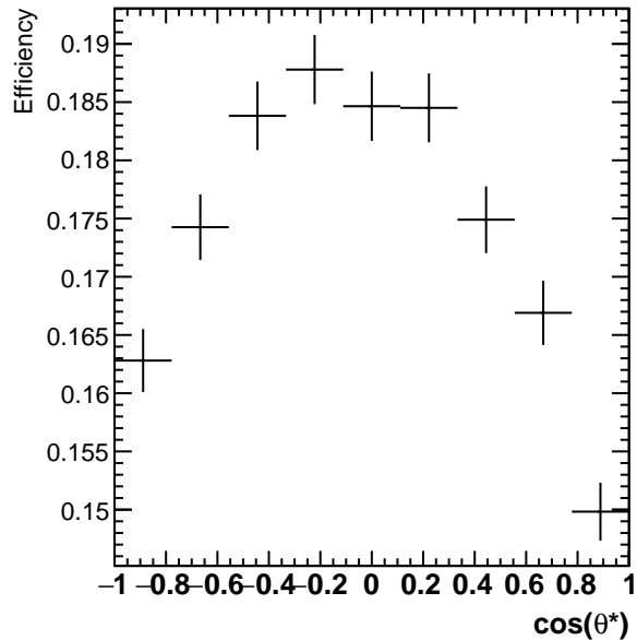
Efficiency 3.0 < p_T < 4.2
