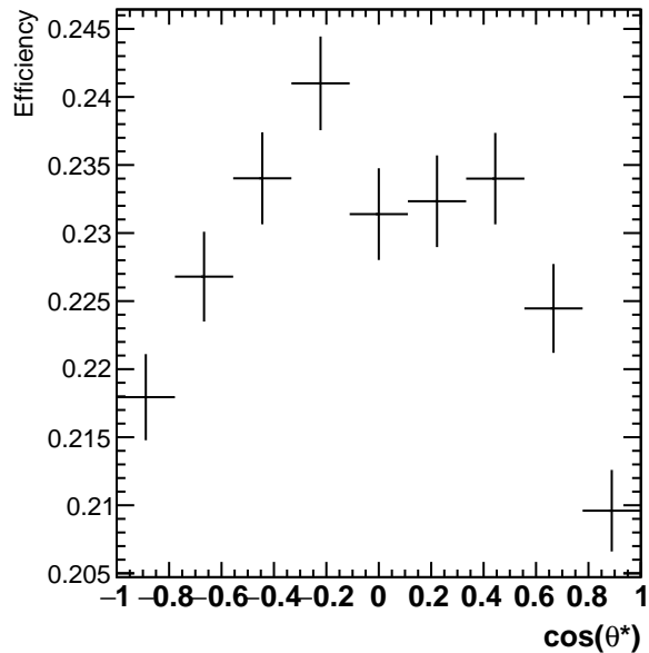
Efficiency 1.8 < p_T < 2.4
