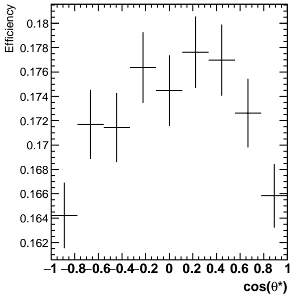
Efficiency 1.2 < p_T < 1.8
