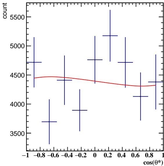
Corrected Yields 2.4 < p_T < 3.0 , 4\pi/6 < \phi' < 5\pi/6
