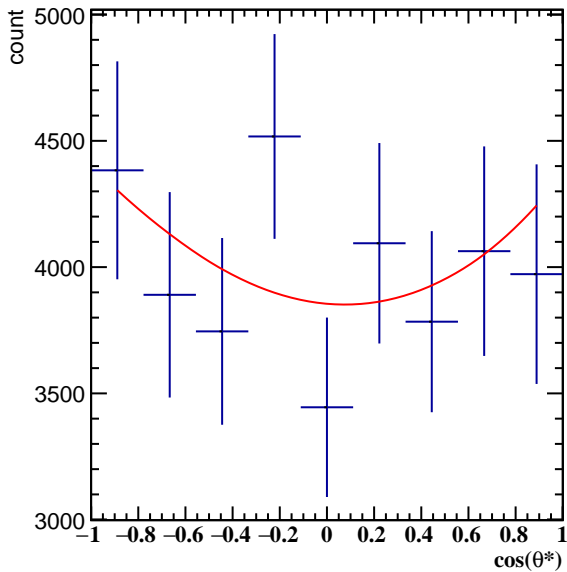
Corrected Yields 2.4 < p_T < 3.0 , 6\pi/6 < \phi' < 7\pi/6
