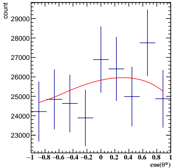
Corrected Yields 1.8 < p_T < 2.4 , 10\pi/6 < \phi' < 11\pi/6
