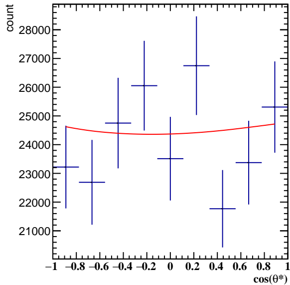
Corrected Yields 1.8 < p_T < 2.4 , 11\pi/6 < \phi' < 12\pi/6
