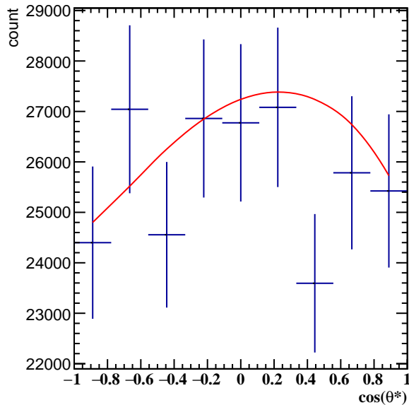
Corrected Yields 1.8 < p_T < 2.4 , 9\pi/6 < \phi' < 10\pi/6
