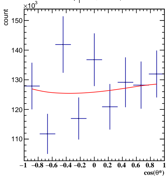
Corrected Yields 1.2 < p_T < 1.8 , 0\pi/6 < \phi' < 1\pi/6
