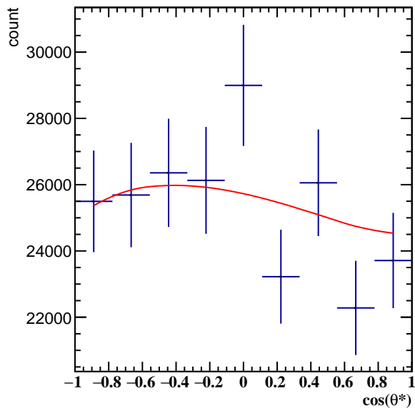
Corrected Yields 1.8 < p_T < 2.4 , 1\pi/6 < \phi' < 2\pi/6
