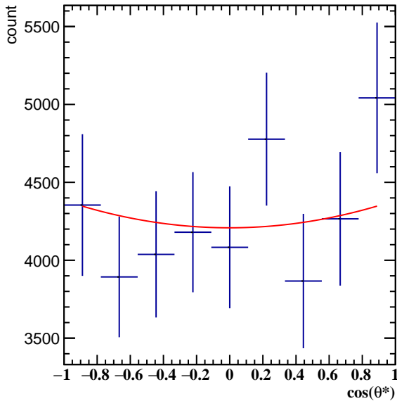
Corrected Yields 2.4 < p_T < 3.0 , 7\pi/6 < \phi' < 8\pi/6
