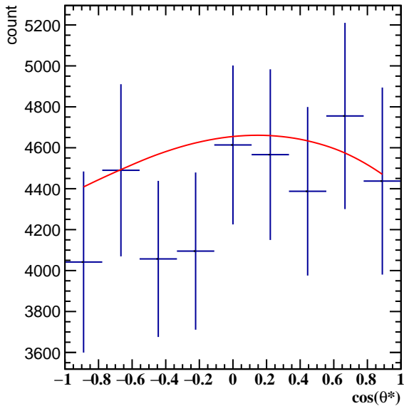
Corrected Yields 2.4 < p_T < 3.0 , 8\pi/6 < \phi' < 9\pi/6
