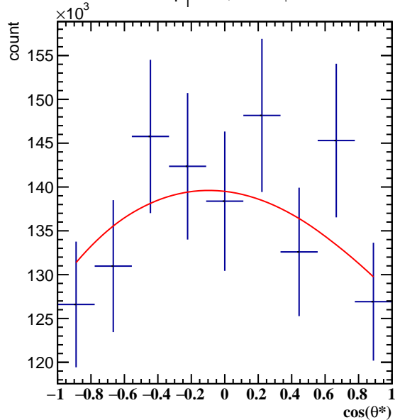
Corrected Yields 1.2 < p_T < 1.8 , 8\pi/6 < \phi' < 9\pi/6
