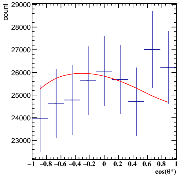
Corrected Yields 1.8 < p_T < 2.4 , 4\pi/6 < \phi' < 5\pi/6
