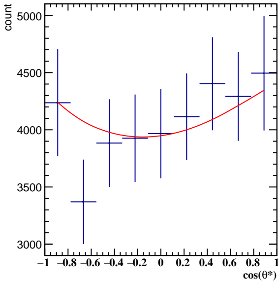
Corrected Yields 2.4 < p_T < 3.0 , 11\pi/6 < \phi' < 12\pi/6
