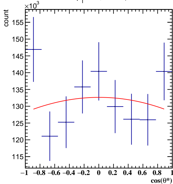
Corrected Yields 1.2 < p_T < 1.8 , 4\pi/6 < \phi' < 5\pi/6
