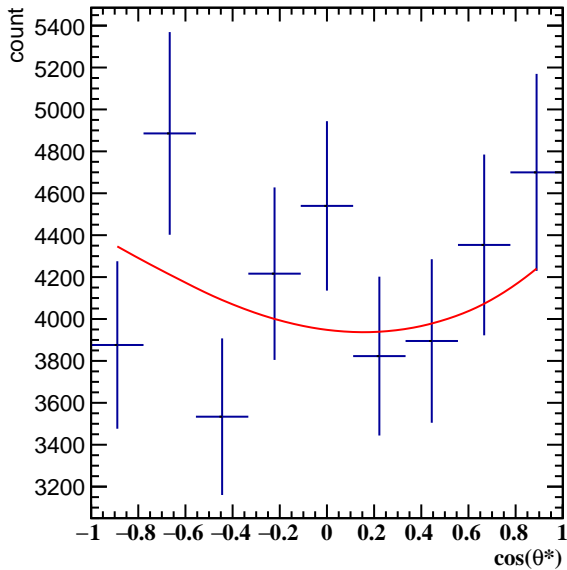
Corrected Yields 2.4 < p_T < 3.0 , 5\pi/6 < \phi' < 6\pi/6
