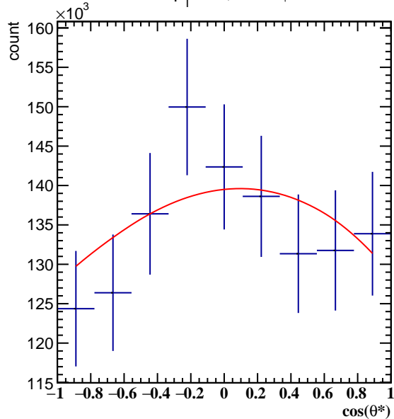
Corrected Yields 1.2 < p_T < 1.8 , 2\pi/6 < \phi' < 3\pi/6
