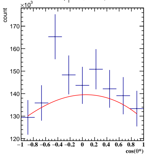
Corrected Yields 1.2 < p_T < 1.8 , 3\pi/6 < \phi' < 4\pi/6
