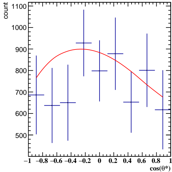
Corrected Yields 3.0 < p_T < 4.2 , 8\pi/6 < \phi' < 9\pi/6
