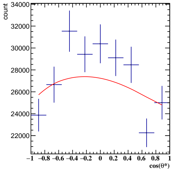
Corrected Yields 1.8 < p_T < 2.4 , 3\pi/6 < \phi' < 4\pi/6
