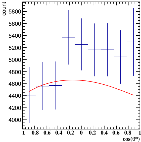
Corrected Yields 2.4 < p_T < 3.0 , 2\pi/6 < \phi' < 3\pi/6
