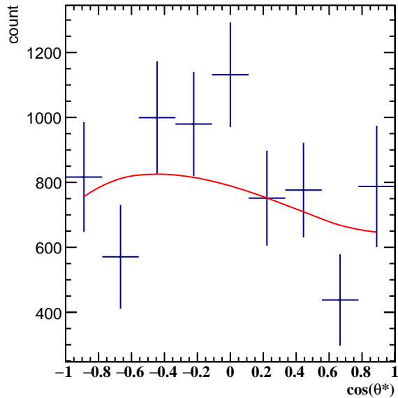
Corrected Yields 3.0 < p_T < 4.2 , 5\pi/6 < \phi' < 6\pi/6
