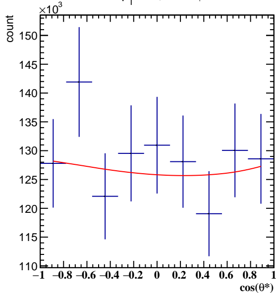
Corrected Yields 1.2 < p_T < 1.8 , 5\pi/6 < \phi' < 6\pi/6
