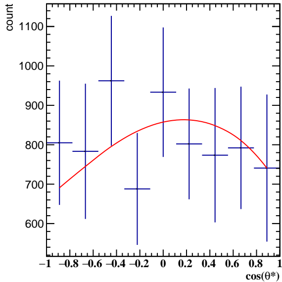
Corrected Yields 3.0 < p_T < 4.2 , 10\pi/6 < \phi' < 11\pi/6
