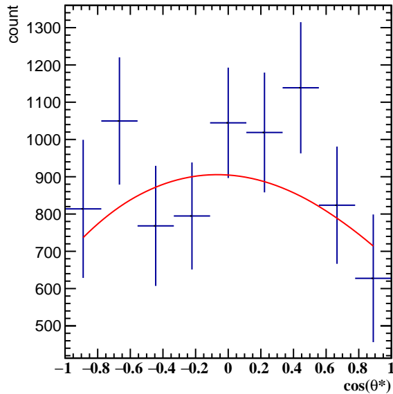
Corrected Yields 3.0 < p_T < 4.2 , 9\pi/6 < \phi' < 10\pi/6
