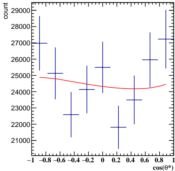
Corrected Yields 1.8 < p_T < 2.4 , 0\pi/6 < \phi' < 1\pi/6
