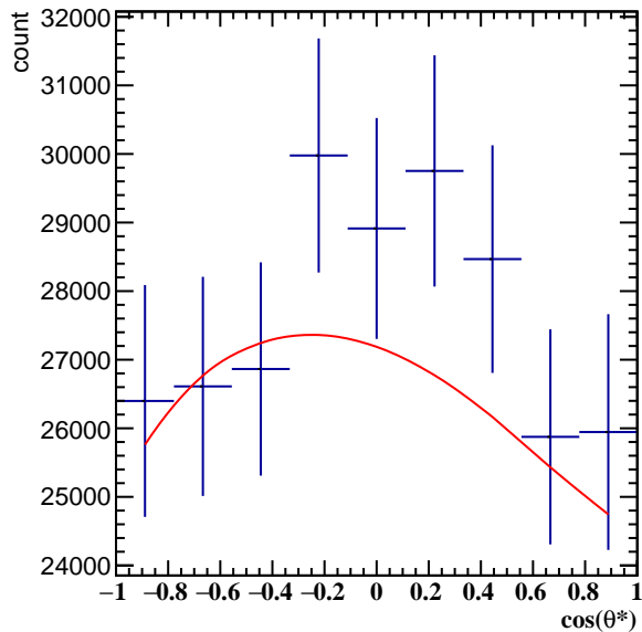
Corrected Yields 1.8 < p_T < 2.4 , 2\pi/6 < \phi' < 3\pi/6
