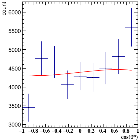
Corrected Yields 2.4 < p_T < 3.0 , 10\pi/6 < \phi' < 11\pi/6
