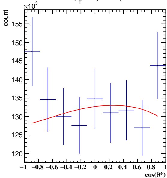
Corrected Yields 1.2 < p_T < 1.8 , 1\pi/6 < \phi' < 2\pi/6
