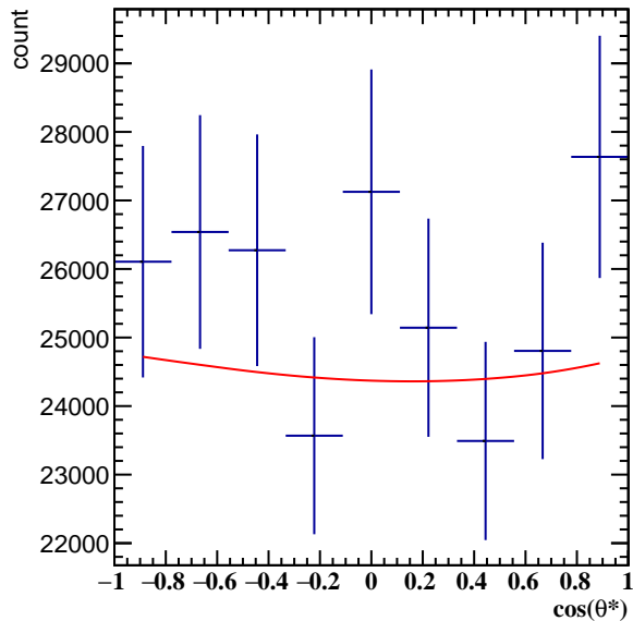
Corrected Yields 1.8 < p_T < 2.4 , 5\pi/6 < \phi' < 6\pi/6
