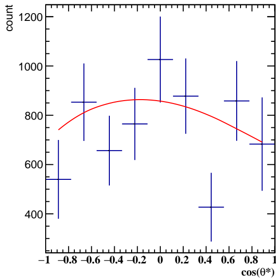
Corrected Yields 3.0 < p_T < 4.2 , 4\pi/6 < \phi' < 5\pi/6
