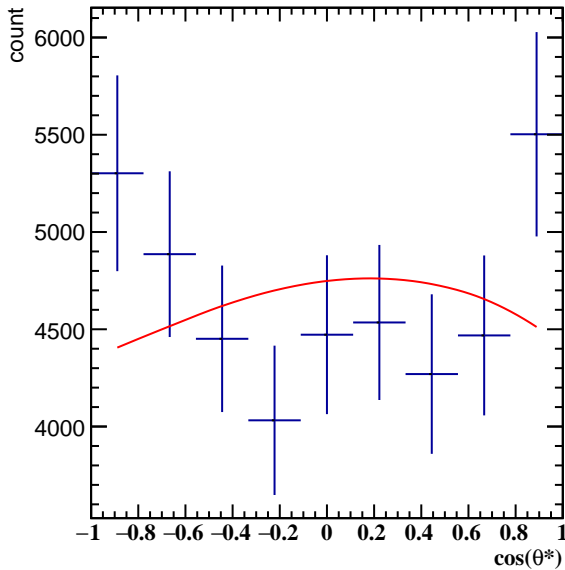
Corrected Yields 2.4 < p_T < 3.0 , 9\pi/6 < \phi' < 10\pi/6
