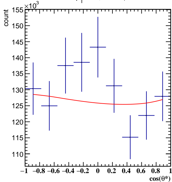
Corrected Yields 1.2 < p_T < 1.8 , 6\pi/6 < \phi' < 7\pi/6
