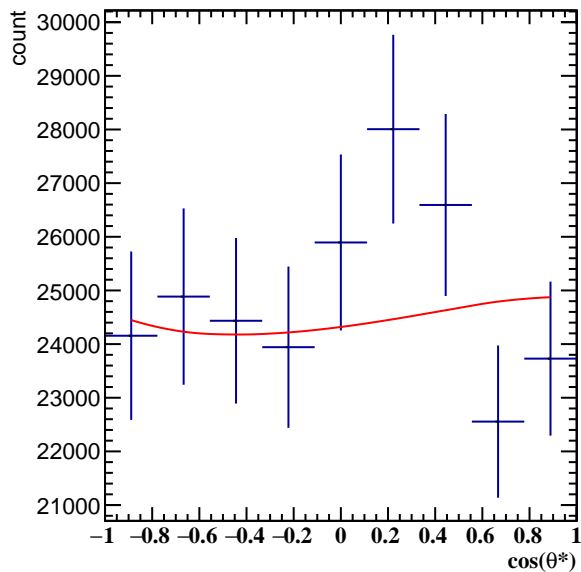
Corrected Yields 1.8 < p_T < 2.4 , 6\pi/6 < \phi' < 7\pi/6
