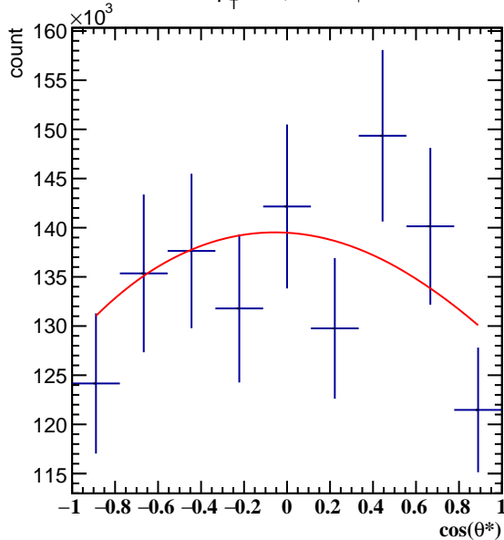
Corrected Yields 1.2 < p_T < 1.8 , 9\pi/6 < \phi' < 10\pi/6
