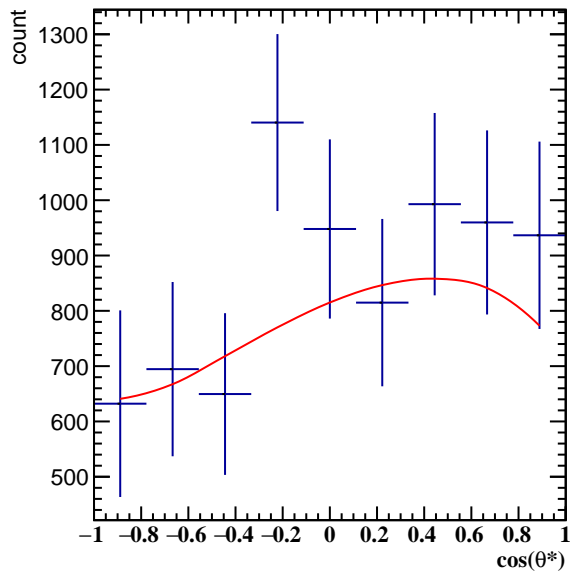
Corrected Yields 3.0 < p_T < 4.2 , 1\pi/6 < \phi' < 2\pi/6
