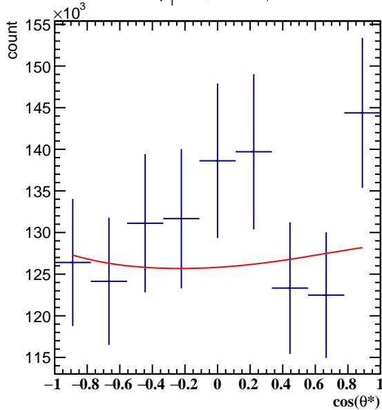
Corrected Yields 1.2 < p_T < 1.8 , 11\pi/6 < \phi' < 12\pi/6
