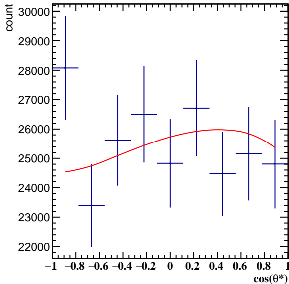
Corrected Yields 1.8 < p_T < 2.4 , 7\pi/6 < \phi' < 8\pi/6
