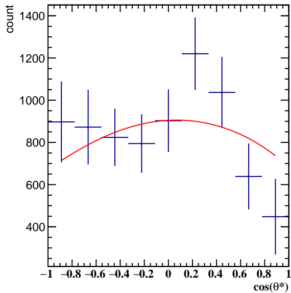
Corrected Yields 3.0 < p_T < 4.2 , 3\pi/6 < \phi' < 4\pi/6
