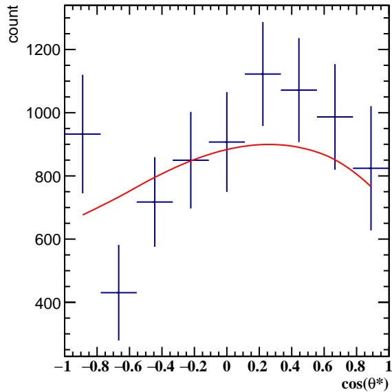
Corrected Yields 3.0 < p_T < 4.2 , 2\pi/6 < \phi' < 3\pi/6
