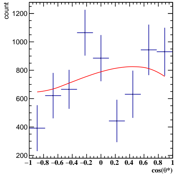
Corrected Yields 3.0 < p_T < 4.2 , 11\pi/6 < \phi' < 12\pi/6
