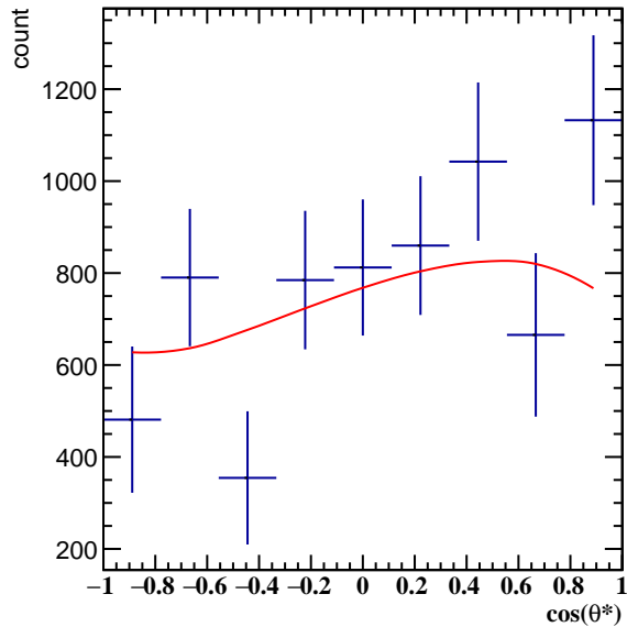
Corrected Yields 3.0 < p_T < 4.2 , 0\pi/6 < \phi' < 1\pi/6
