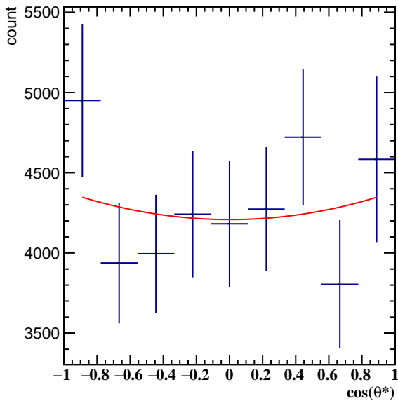
Corrected Yields 2.4 < p_T < 3.0 , 1\pi/6 < \phi' < 2\pi/6
