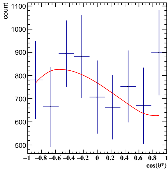
Corrected Yields 3.0 < p_T < 4.2 , 6\pi/6 < \phi' < 7\pi/6
