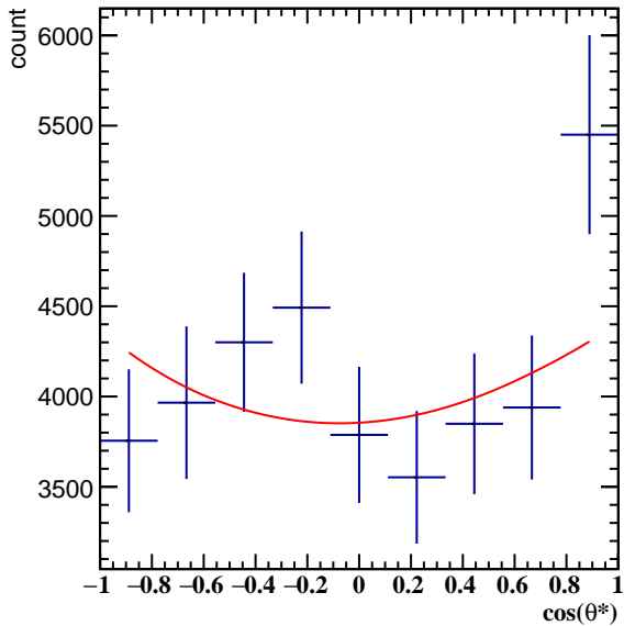
Corrected Yields 2.4 < p_T < 3.0 , 0\pi/6 < \phi' < 1\pi/6
