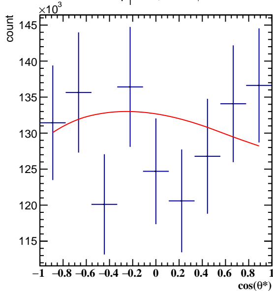
Corrected Yields 1.2 < p_T < 1.8 , 7\pi/6 < \phi' < 8\pi/6
