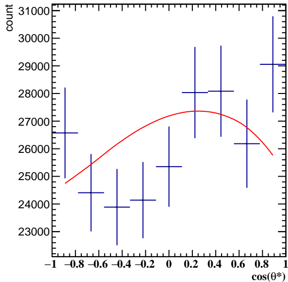
Corrected Yields 1.8 < p_T < 2.4 , 8\pi/6 < \phi' < 9\pi/6
