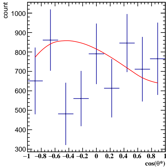
Corrected Yields 3.0 < p_T < 4.2 , 7\pi/6 < \phi' < 8\pi/6
