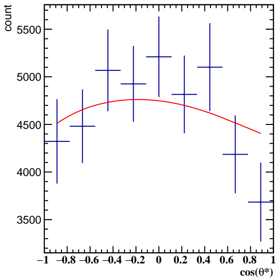
Corrected Yields 2.4 < p_T < 3.0 , 3\pi/6 < \phi' < 4\pi/6
