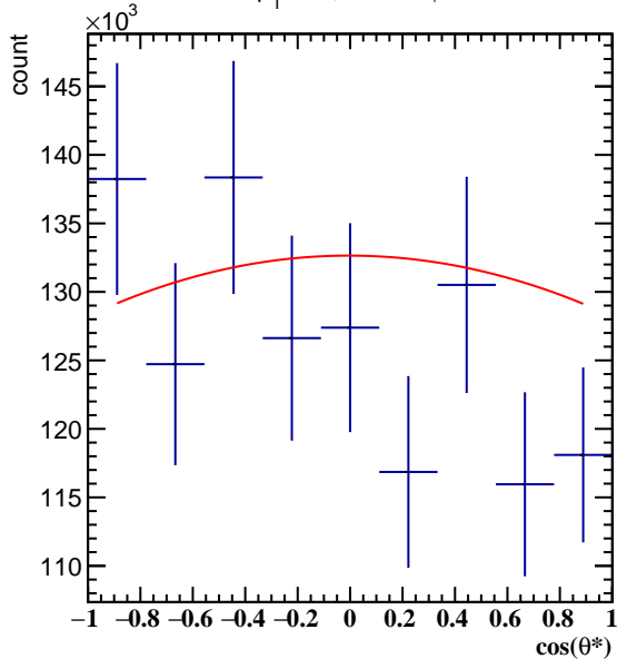
Corrected Yields 1.2 < p_T < 1.8 , 10\pi/6 < \phi' < 11\pi/6
