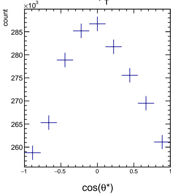
Raw Yields 1.2 < p_T < 1.8
