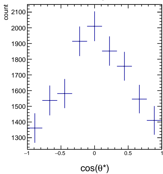
Raw Yields 3.0 < p_T < 4.2
