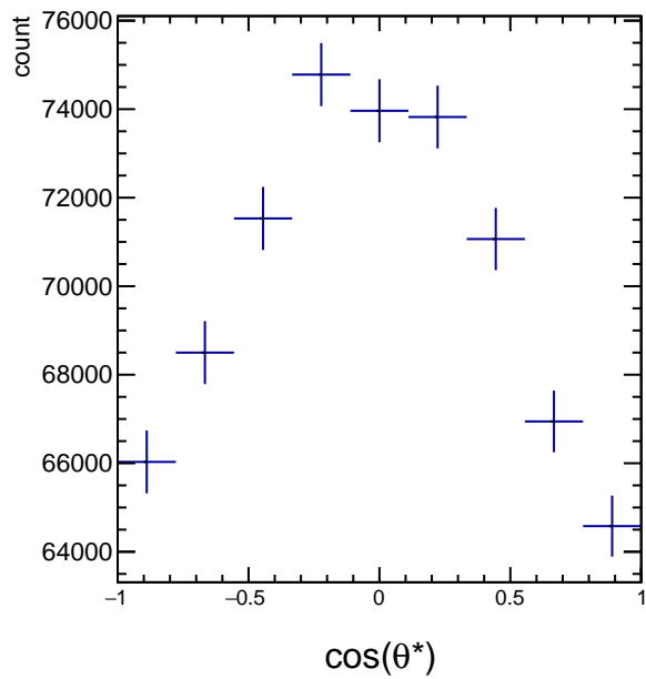
Raw Yields 1.8 < p_T < 2.4
