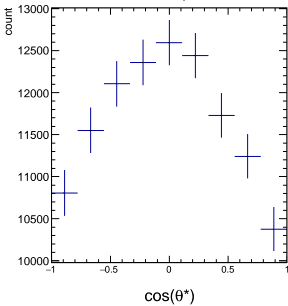
Raw Yields 2.4 < p_T < 3.0
