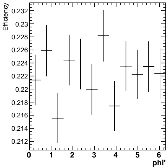
Efficiency 2.4 < p_T < 3.0
