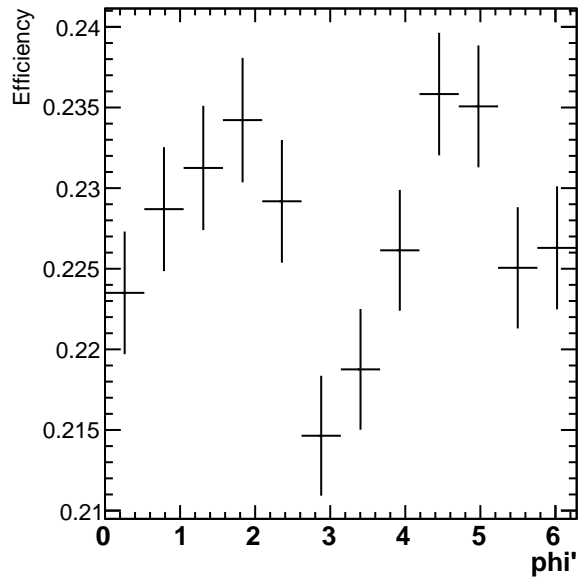
Efficiency 1.8 < p_T < 2.4
