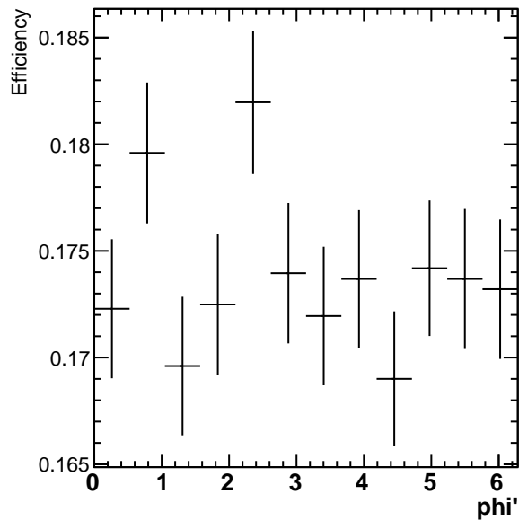
Efficiency 3.0 < p_T < 4.2
