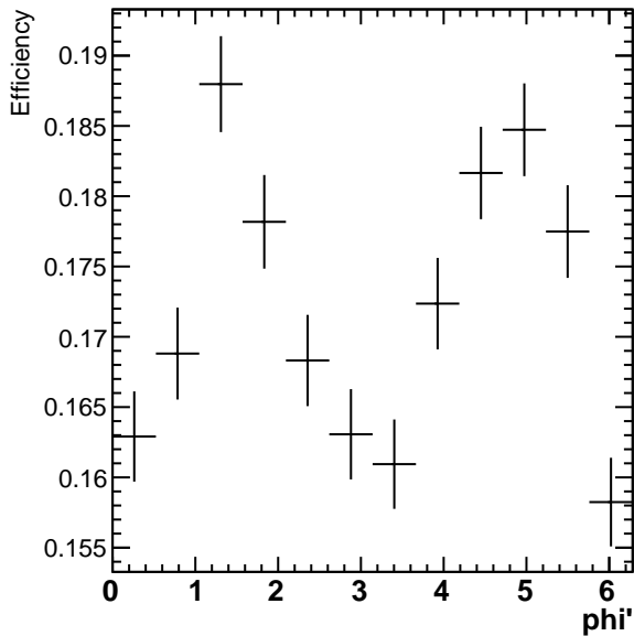
Efficiency 1.2 < p_T < 1.8
