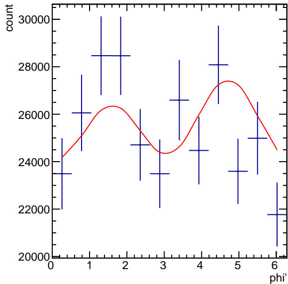
Corrected Yields 1.8 < p_T < 2.4 , 1.5/4.5 < \cos(\theta^*) < 2.5/4.5
