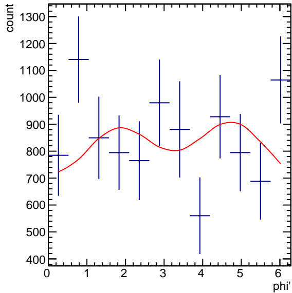
Corrected Yields 3.0 < p_T < 4.2, -1.5/4.5 < \cos(\theta^*) < -0.5/4.5
