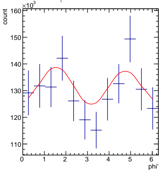
Corrected Yields 1.2 < p_T < 1.8 , 1.5/4.5 < \cos(\theta^*) < 2.5/4.5
