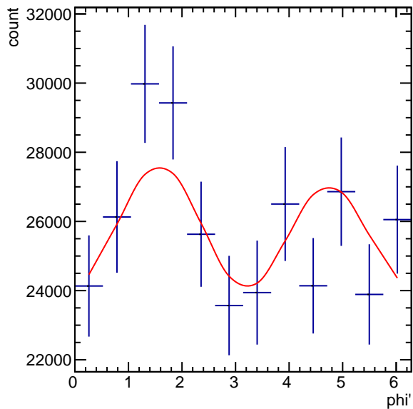
Corrected Yields 1.8 < p_T < 2.4, -1.5/4.5 < \cos(\theta^*) < -0.5/4.5
