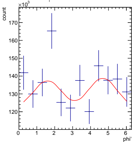
Corrected Yields 1.2 < p_T < 1.8, -2.5/4.5 < \cos(\theta^*) < -1.5/4.5
