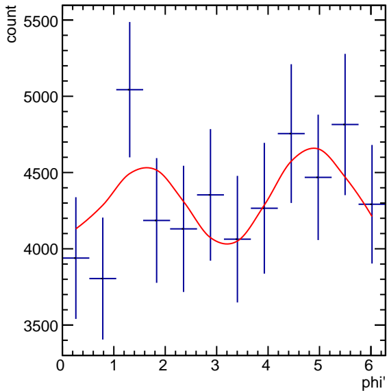
Corrected Yields 2.4 < p_T < 3.0, 2.5/4.5 < \cos(\theta^*) < 3.5/4.5
