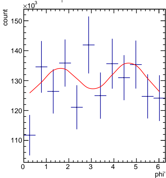
Corrected Yields 1.2 < p_T < 1.8 , -3.5/4.5 < \cos(\theta^*) < -2.5/4.5
