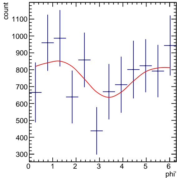
Corrected Yields 3.0 < p_T < 4.2, 2.5/4.5 < \cos(\theta^*) < 3.5/4.5
