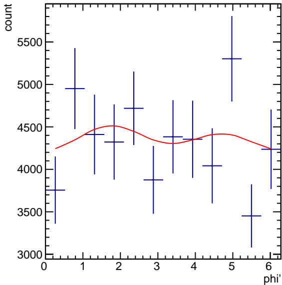
Corrected Yields 2.4 < p_T < 3.0 , -4.5/4.5 < \cos(\theta^*) < -3.5/4.5
