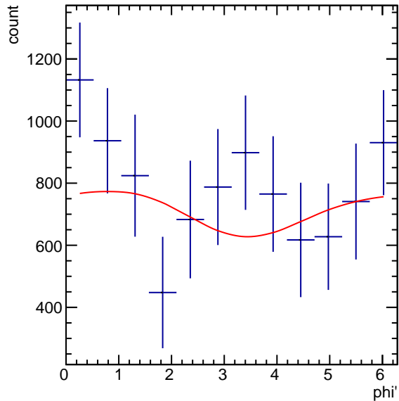
Corrected Yields 3.0 < p_T < 4.2, 3.5/4.5 < \cos(\theta^*) < 4.5/4.5
