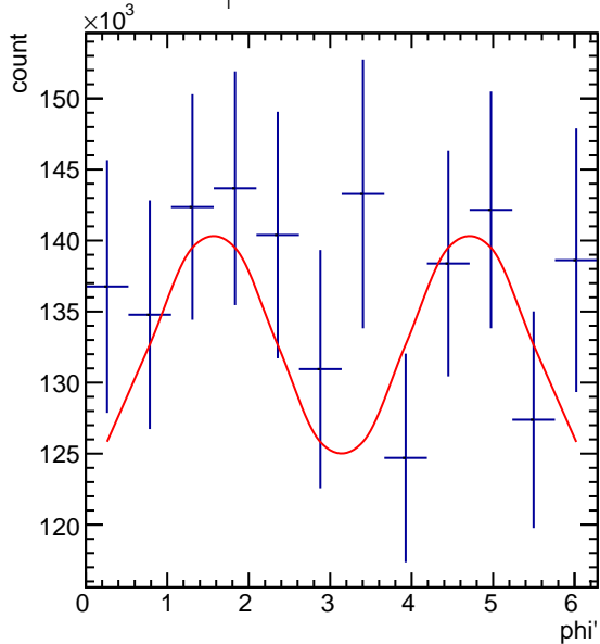
Corrected Yields 1.2 < p_T < 1.8, -0.5/4.5 < \cos(\theta^*) < 0.5/4.5
