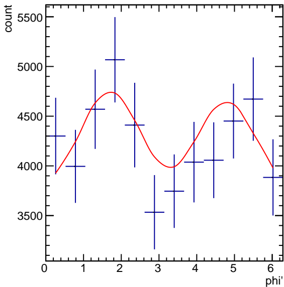
Corrected Yields 2.4 < p_T < 3.0, -2.5/4.5 < \cos(\theta^*) < -1.5/4.5
