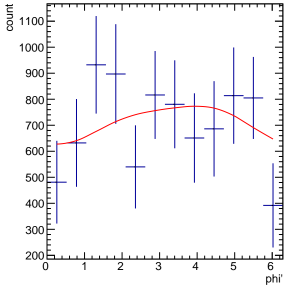
Corrected Yields 3.0 < p_T < 4.2 , -4.5/4.5 < \cos(\theta^*) < -3.5/4.5
