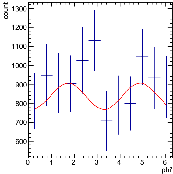
Corrected Yields 3.0 < p_T < 4.2, -0.5/4.5 < \cos(\theta^*) < 0.5/4.5
