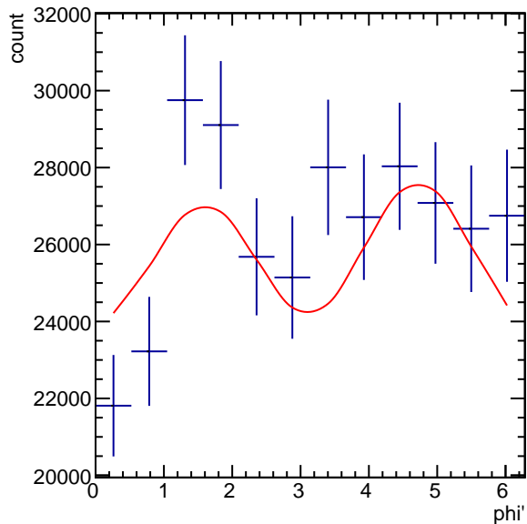
Corrected Yields 1.8 < p_T < 2.4 , 0.5/4.5 < \cos(\theta^*) < 1.5/4.5
