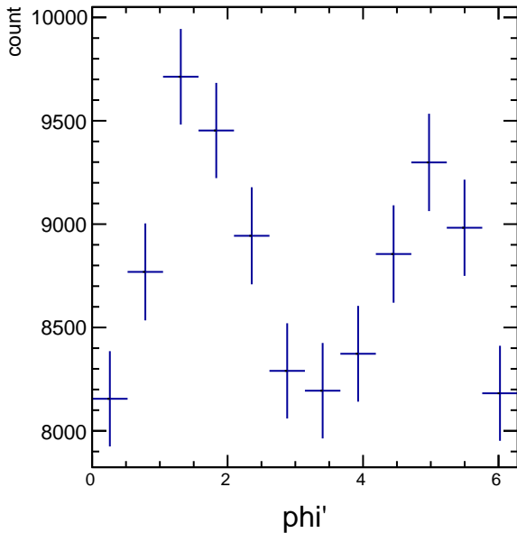
Raw Yields 2.4 < p_T < 3.0
