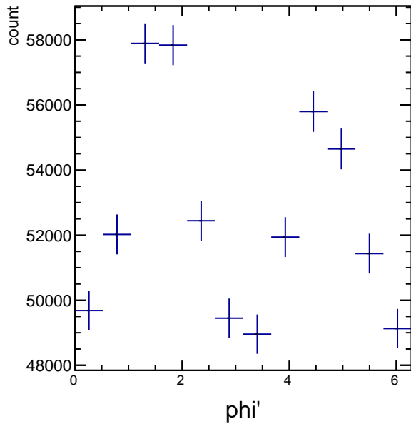
Raw Yields 1.8 < p_T < 2.4
