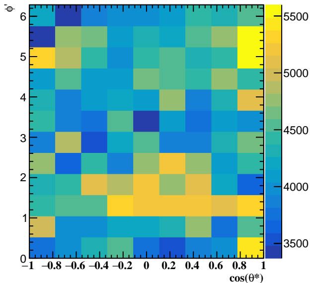
Corrected Yields 2.4 < p_T < 3.0
