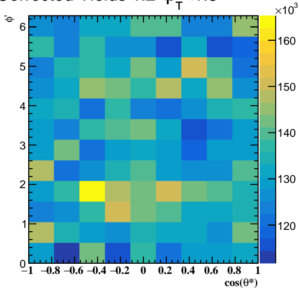
Corrected Yields 1.2 < p_T < 1.8
