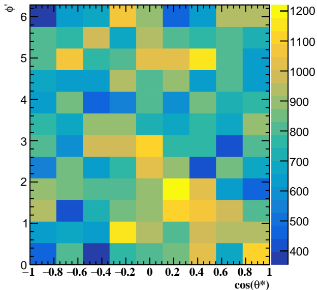
Corrected Yields 3.0 < p_T < 4.2
