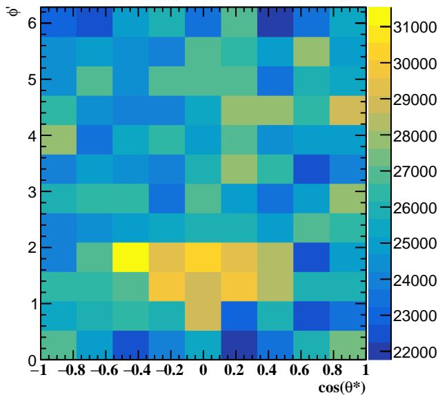
Corrected Yields 1.8 < p_T < 2.4
