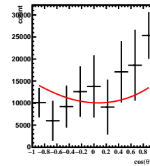
Corrected Yields 4/5 < y < 5/5 , 5\pi/6 < \phi' < 6\pi/6
