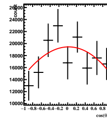
Corrected Yields 4/5 < y < 5/5 , 3\pi/6 < \phi' < 4\pi/6
