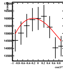
Corrected Yields -3/5 < y < -2/5 , 6\pi/6 < \phi' < 7\pi/6
