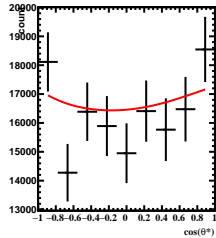
Corrected Yields -4/5 < y < -3/5 , 1\pi/6 < \phi' < 2\pi/6
