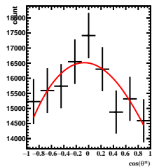
Corrected Yields 1/5 < y < 2/5 , 11\pi/6 < \phi < 12\pi/6
