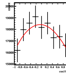
Corrected Yields 3/5 < y < 4/5 , 3\pi/6 < \phi' < 4\pi/6
