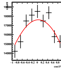
Corrected Yields -2/5 < y < -1/5 , 2\pi/6 < \phi' < 3\pi/6
