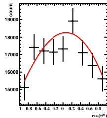
Corrected Yields -1/5 < y < 0/5 , 9\pi/6 < \phi' < 10\pi/6
