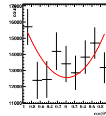
Corrected Yields 3/5 < y < 4/5 , 0\pi/6 < \phi' < 1\pi/6
