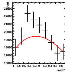
Corrected Yields -4/5 < y < -3/5 , 3\pi/6 < \phi' < 4\pi/6
