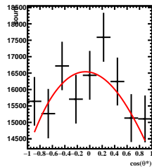
Corrected Yields 1/5 < y < 2/5 , 0\pi/6 < \phi' < 1\pi/6
