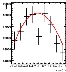
Corrected Yields 0/5 < y < 1/5 , 9\pi/6 < \phi' < 10\pi/6
