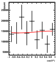
Corrected Yields 4/5 < y < 5/5 , 1\pi/6 < \phi' < 2\pi/6
