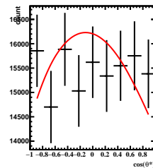
Corrected Yields 2/5 < y < 3/5 , 1\pi/6 < \phi' < 2\pi/6
