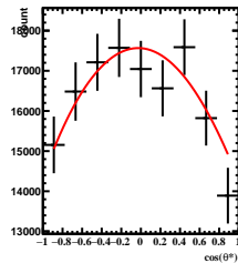
Corrected Yields -2/5 < y < -1/5 , 9\pi/6 < \phi' < 10\pi/6
