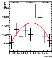
Corrected Yields 0/5 < y < 1/5 , 4\pi/6 < \phi' < 5\pi/6
