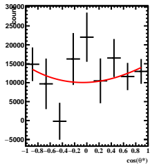
Corrected Yields 4/5 < y < 5/5 , 11\pi/6 < \phi < 12\pi/6
