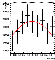
Corrected Yields 4/5 < y < 5/5 , 9\pi/6 < \phi' < 10\pi/6
