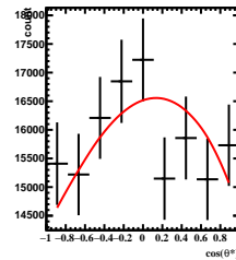
Corrected Yields -3/5 < y < -2/5 , 1\pi/6 < \phi' < 2\pi/6
