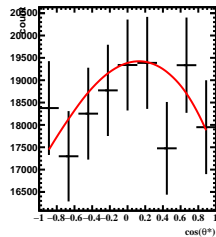
Corrected Yields -4/5 < y < -3/5 , 9\pi/6 < \phi' < 10\pi/6
