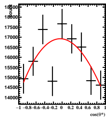
Corrected Yields 1/5 < y < 2/5 , 1\pi/6 < \phi' < 2\pi/6
