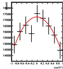
Corrected Yields 1/5 < y < 2/5 , 9\pi/6 < \phi' < 10\pi/6
