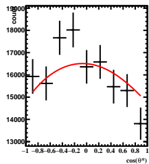
Corrected Yields 0/5 < y < 1/5 , 11\pi/6 < \phi < 12\pi/6
