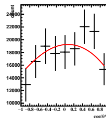
Corrected Yields 4/5 < y < 5/5 , 2\pi/6 < \phi' < 3\pi/6
