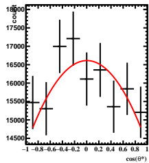
Corrected Yields -2/5 < y < -1/5 , 11\pi/6 < \phi < 12\pi/6
