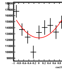
Corrected Yields 3/5 < y < 4/5 , 5\pi/6 < \phi' < 6\pi/6
