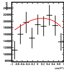
Corrected Yields -5/5 < y < -4/5 , 8\pi/6 < \phi' < 9\pi/6
