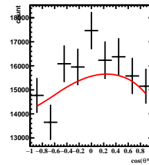
Corrected Yields 2/5 < y < 3/5 , 5\pi/6 < \phi' < 6\pi/6
