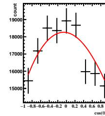
Corrected Yields -1/5 < y < 0/5 , 3\pi/6 < \phi' < 4\pi/6
