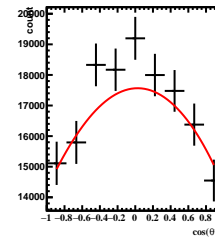
Corrected Yields -2/5 < y < -1/5 , 3\pi/6 < \phi' < 4\pi/6
