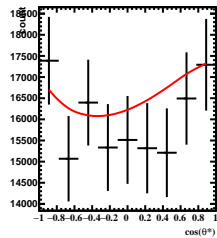
Corrected Yields -4/5 < y < -3/5 , 10\pi/6 < \phi < 11\pi/6
