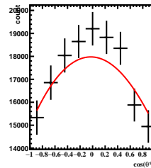
Corrected Yields -1/5 < y < 0/5 , 2\pi/6 < \phi' < 3\pi/6
