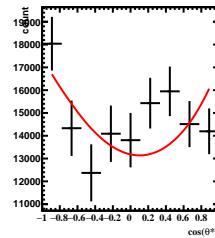
Corrected Yields -4/5 < y < -3/5 , 5\pi/6 < \phi' < 6\pi/6
