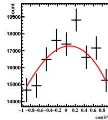
Corrected Yields -3/5 < y < -2/5 , 2\pi/6 < \phi' < 3\pi/6
