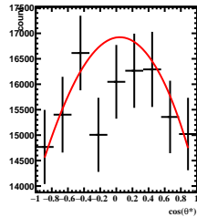
Corrected Yields 1/5 < y < 2/5 , 7\pi/6 < \phi' < 8\pi/6
