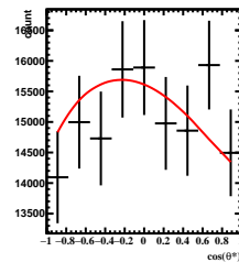
Corrected Yields 2/5 < y < 3/5 , 0\pi/6 < \phi' < 1\pi/6
