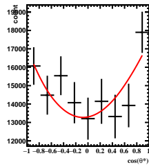
Corrected Yields -4/5 < y < -3/5 , 0\pi/6 < \phi' < 1\pi/6
