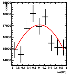
Corrected Yields -2/5 < y < -1/5 , 4\pi/6 < \phi' < 5\pi/6
