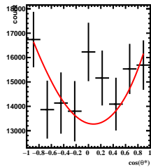
Corrected Yields -4/5 < y < -3/5 , 6\pi/6 < \phi' < 7\pi/6
