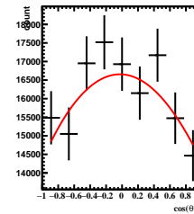
Corrected Yields -2/5 < y < -1/5 , 6\pi/6 < \phi' < 7\pi/6
