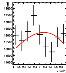
Corrected Yields -1/5 < y < 0/5 , 0\pi/6 < \phi' < 1\pi/6
