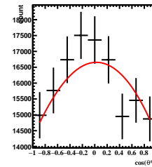
Corrected Yields -2/5 < y < -1/5 , 0\pi/6 < \phi' < 1\pi/6
