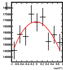
Corrected Yields 1/5 < y < 2/5 , 10\pi/6 < \phi < 11\pi/6
