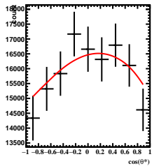
Corrected Yields -1/5 < y < 0/5 , 11\pi/6 < \phi < 12\pi/6
