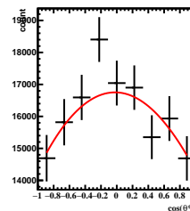
Corrected Yields 2/5 < y < 3/5 , 2\pi/6 < \phi' < 3\pi/6
