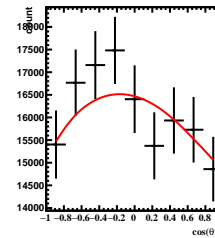
Corrected Yields -1/5 < y < 0/5 , 5\pi/6 < \phi' < 6\pi/6
