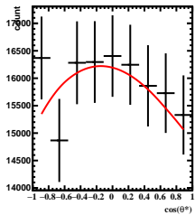
Corrected Yields -1/5 < y < 0/5 , 6\pi/6 < \phi' < 7\pi/6
