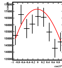
Corrected Yields -2/5 < y < -1/5 , 7\pi/6 < \phi' < 8\pi/6
