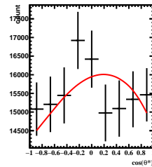
Corrected Yields -3/5 < y < -2/5 , 0\pi/6 < \phi' < 1\pi/6
