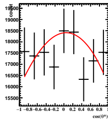
Corrected Yields 3/5 < y < 4/5 , 9\pi/6 < \phi' < 10\pi/6
