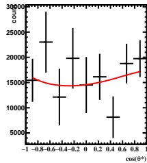
Corrected Yields -5/5 < y < -4/5 , 7\pi/6 < \phi' < 8\pi/6
