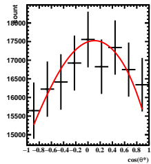
Corrected Yields -1/5 < y < 0/5 , 10\pi/6 < \phi < 11\pi/6
