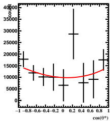
Corrected Yields 4/5 < y < 5/5 , 6\pi/6 < \phi' < 7\pi/6
