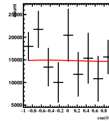
Corrected Yields 4/5 < y < 5/5 , 4\pi/6 < \phi' < 5\pi/6
