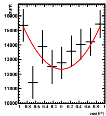
Corrected Yields 3/5 < y < 4/5 , 11\pi/6 < \phi < 12\pi/6
