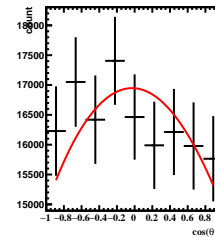
Corrected Yields -1/5 < y < 0/5 , 7\pi/6 < \phi' < 8\pi/6
