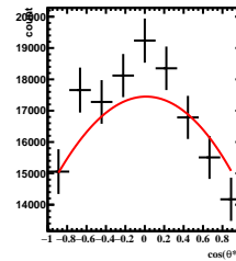
Corrected Yields -3/5 < y < -2/5 , 3\pi/6 < \phi' < 4\pi/6
