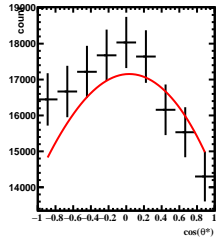
Corrected Yields -2/5 < y < -1/5 , 1\pi/6 < \phi' < 2\pi/6
