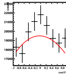
Corrected Yields -4/5 < y < -3/5 , 2\pi/6 < \phi' < 3\pi/6
