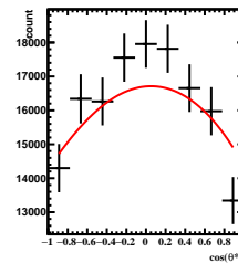
Corrected Yields 2/5 < y < 3/5 , 3\pi/6 < \phi' < 4\pi/6
