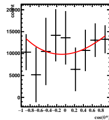
Corrected Yields 4/5 < y < 5/5 , 0\pi/6 < \phi' < 1\pi/6
