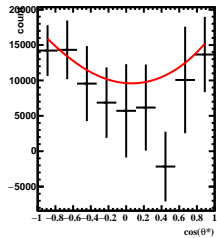
Corrected Yields -5/5 < y < -4/5 , 11\pi/6 < \phi < 12\pi/6
