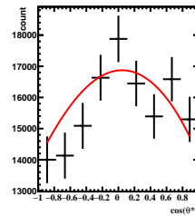
Corrected Yields 1/5 < y < 2/5 , 4\pi/6 < \phi' < 5\pi/6
