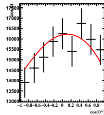
Corrected Yields 2/5 < y < 3/5 , 7\pi/6 < \phi' < 8\pi/6
