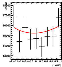
Corrected Yields 3/5 < y < 4/5 , 10\pi/6 < \phi < 11\pi/6
