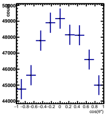
Raw Yields 2/5 < y < 3/5
