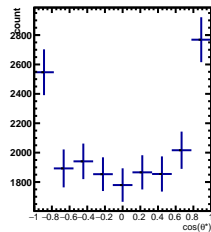
Raw Yields 4/5 < y < 5/5
