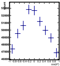
Raw Yields -3/5 < y < -2/5
