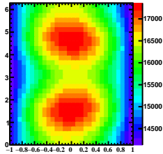
SpinDensity2Dcos
