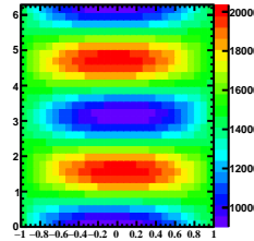
SpinDensity2Dcos
