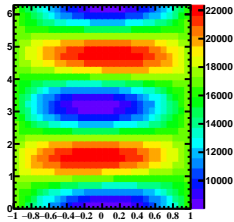
SpinDensity2Dcos
