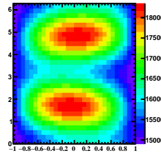
SpinDensity2Dcos
