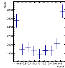
Raw Yields 4/5 < y < 5/5
