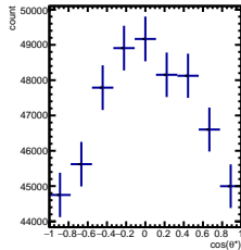
Raw Yields 2/5 < y < 3/5
