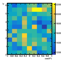
Corrected Yields -3/5 < y < -2/5
