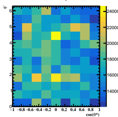
Corrected Yields 0/5 < y < 1/5
