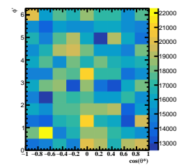
Corrected Yields -2/5 < y < -1/5
