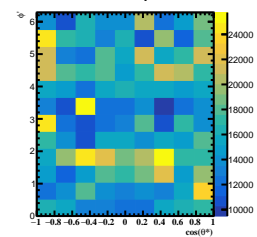
Corrected Yields 3/5 < y < 4/5
