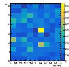
Corrected Yields 4/5 < y < 5/5
