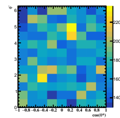
Corrected Yields -1/5 < y < 0/5
