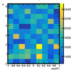
Corrected Yields 1/5 < y < 2/5
