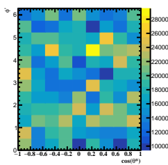
Corrected Yields -4/5 < y < -3/5
