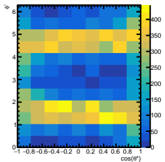
Raw Yields 4/5 < y < 5/5
