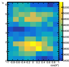
Raw Yields -3/5 < y < -2/5
