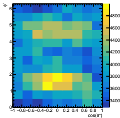
Raw Yields 2/5 < y < 3/5
