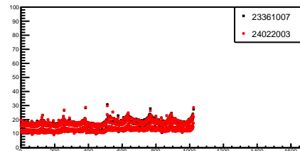
g_ranStdDev_15_1
