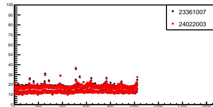
g_ranStdDev_23_0
