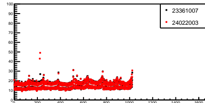
g_ranStdDev_13_1
