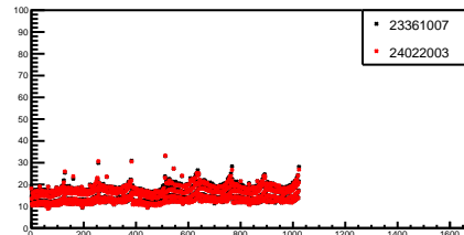
g_ranStdDev_17_1
