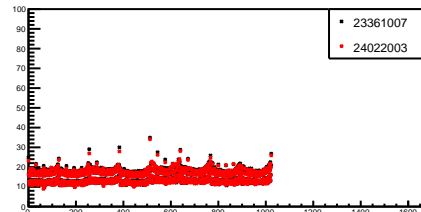
g_ranStdDev_22_0
