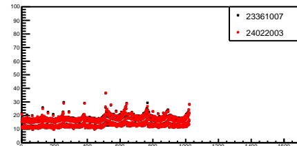
g_ranStdDev_7_1
