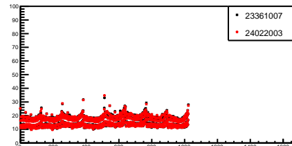
g_ranStdDev_14_1
