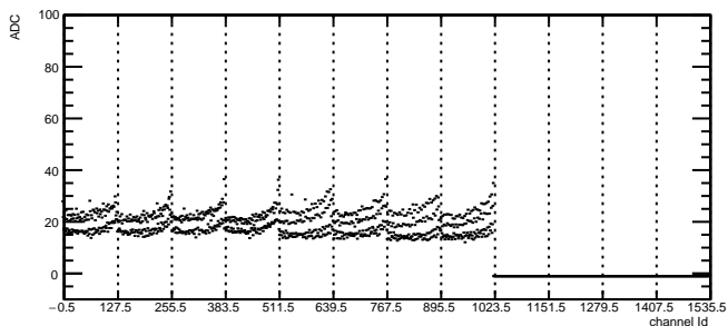
Total Noise: RDO6 Module11 TB0
