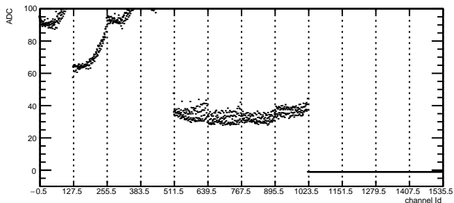
Total Noise: RDO5 Module5 TB2
