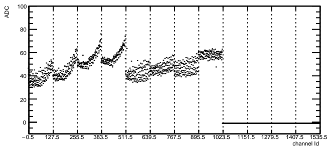
Total Noise: RDO6 Module9 TB0
