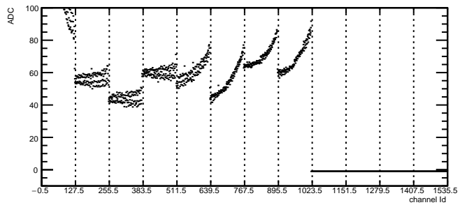
Total Noise: RDO5 Module4 TB1
