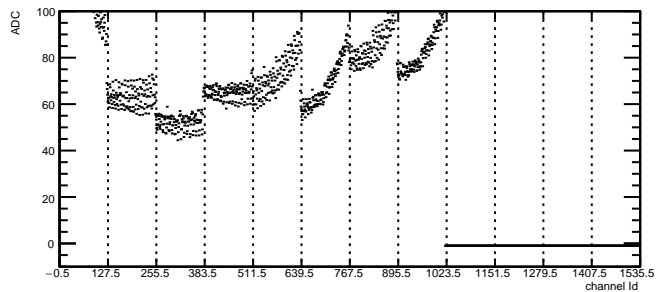
Total Noise: RDO5 Module4 TB0
