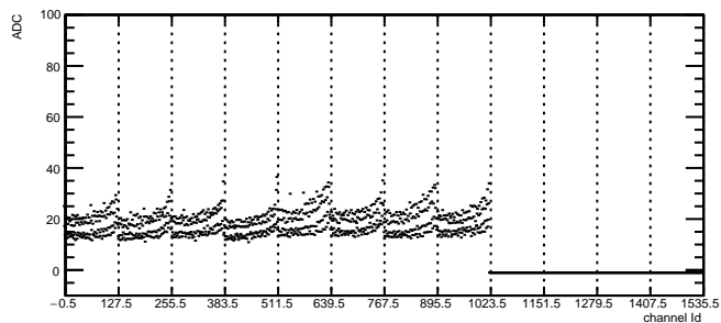
Total Noise: RDO3 Module6 TB1
