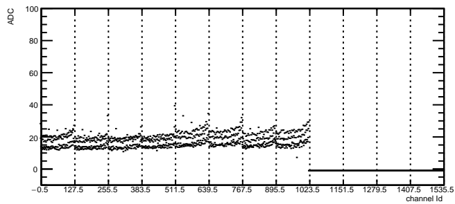
Total Noise: RDO3 Module4 TB1
