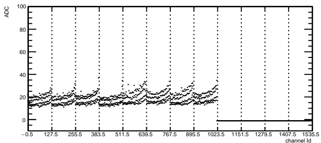
Total Noise: RDO3 Module5 TB1
