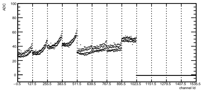
Total Noise: RDO6 Module9 TB2
