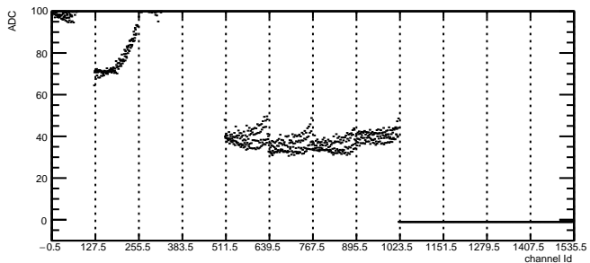
Total Noise: RDO5 Module5 TB1
