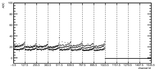
Total Noise: RDO6 Module11 TB2
