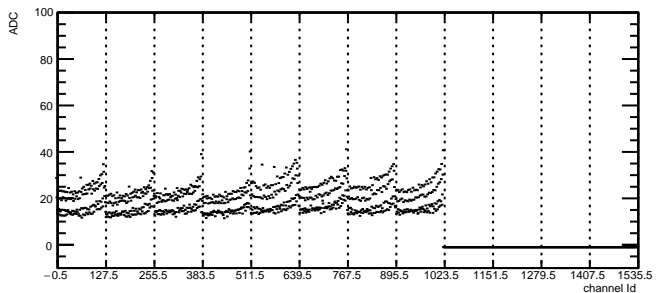
Total Noise: RDO4 Module11 TB1
