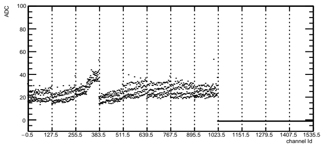
Total Noise: RDO1 Module5 TB2
