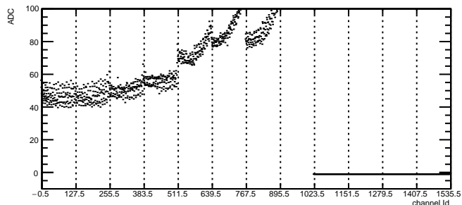
Total Noise: RDO5 Module6 TB0
