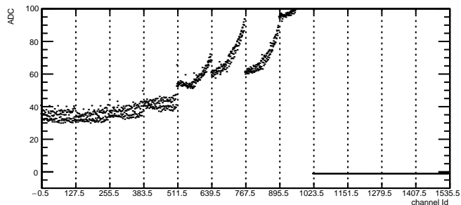
Total Noise: RDO5 Module6 TB2
