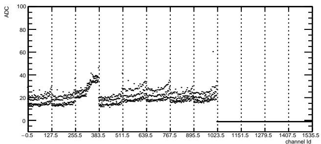
Total Noise: RDO1 Module5 TB1
