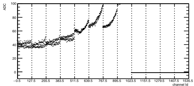
Total Noise: RDO5 Module6 TB1
