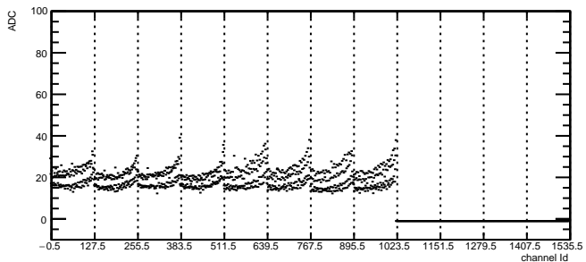
Total Noise: RDO6 Module11 TB1
